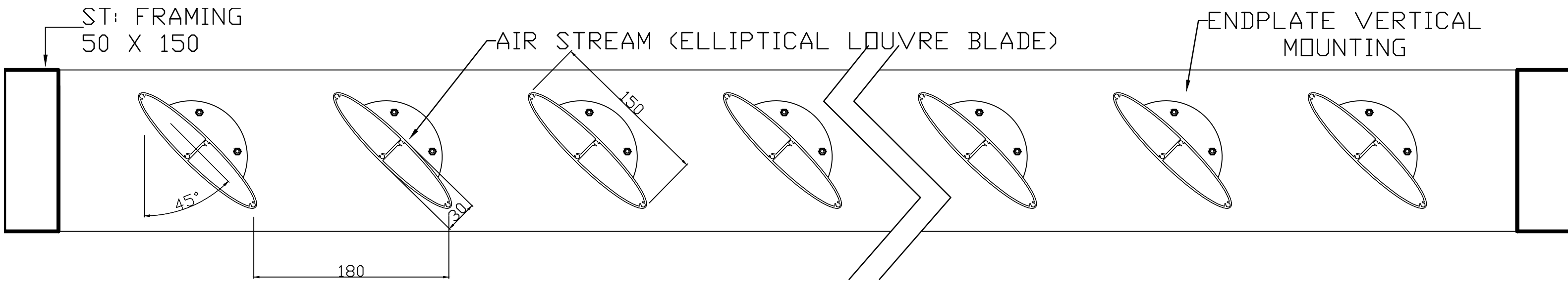
TYPICAL SECTION THROUGH SOLAR SHADE HORIZONTAL VIEW
